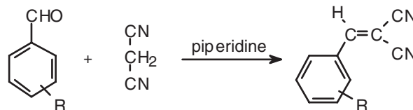
Sch. 1. Monomer synthesis (where R is 2,4-( \text{CH}_3 ) 2 , 2,5-( \text{CH}_3 ) 2 , 3,5-( \text{CH}_3 ) 2 , 3- \text{CH}_3 -4- \text{CH}_3\text{O} , 3- \text{C}_2\text{H}_5 -4- \text{CH}_3\text{O} , 2,4,6-( \text{CH}_3 ) 3 , 2,3-( \text{CH}_3 ) 2 -4- \text{CH}_3\text{O} ).
